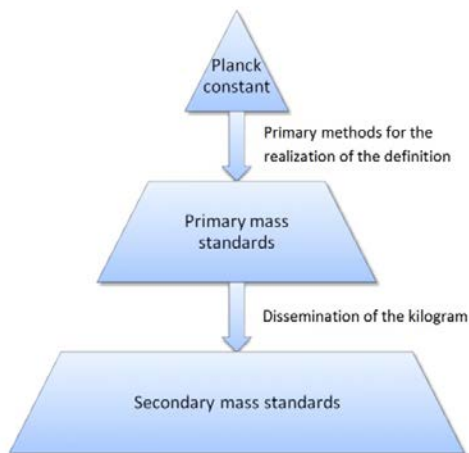
Figure 4. Proposed future realization of the kilogram with primary methods that would link primary mass standards to the fundamental constant h , followed by the classical way of dissemination using the primary mass standards to calibrate secondary ones.
