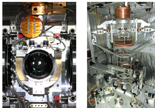
Figure 5. Existing primary methods for the realization of the new kilogram are the “Avogadro method” (or “X-ray Crystal Density (XRCD) method”) and the “Watt balance method”. Left: View of a single crystal silicon sphere. The diameter of the sphere (about 90 mm), and hence, its volume is measured with a Fizeau interferometer, which forms part of the XRCD method (source: PTB Braunschweig, Germany). Right: View into the BIPM watt balance [6].
