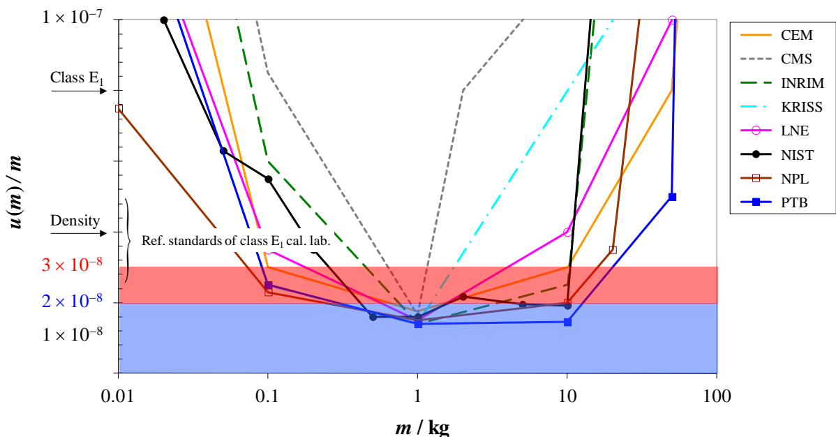
Figure 7. Calibration and Measurement Capabilities (CMCs) for mass standards in the range from 10 g to 100 kg of eight selected NMIs [14] compared with different uncertainty limits for the realization of a redefined kilogram and relative standard uncertainties of the best primary density standards (see pointer "Density"), for reference standards of class E_1 calibration laboratories (see range indicated), and for class E_1 weights (see pointer "Class E_1 ").
