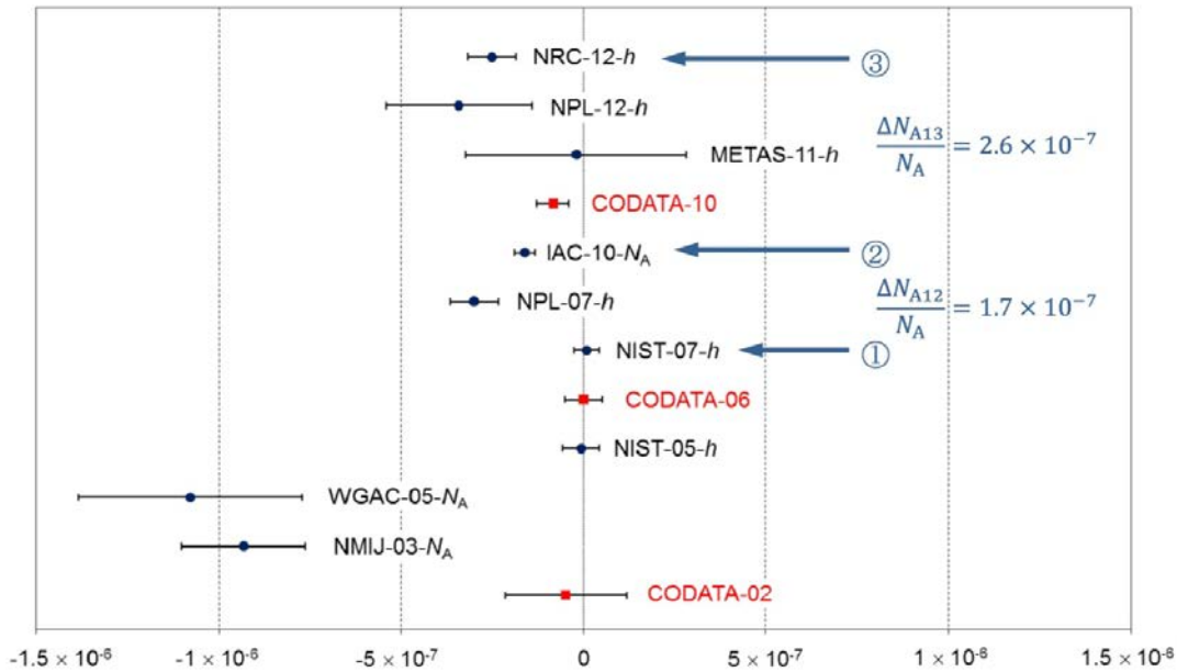
Figure 6. Measurement results for the Avogadro constant N_A with standard uncertainties ( k = 1 ), represented as relative deviations from the CODATA 2006 value ( N_A = 6.02214179(30) \times 10^{23} \text{ mol}^{-1} ). The results for the Planck constant, h , (watt balance) and for K_J (voltage balance) have been converted by means of the CODATA 2006 constants. Explanations: "NPL-07- h ", for example, means: NPL's result in 2007 for a measurement of h . WGAC: Working Group Avogadro Constant, IAC: International Avogadro Coordination. Currently, the three results with the smallest uncertainties are: (1) NIST-07- h ( u_r = 3.6 \times 10^{-8} ), (2) IAC-10- N_A ( u_r = 3.0 \times 10^{-8} ) and (3) NRC-12- h ( u_r = 6.5 \times 10^{-8} ). Measurement results and CODATA values according to the data published in [5, 12, 13].
