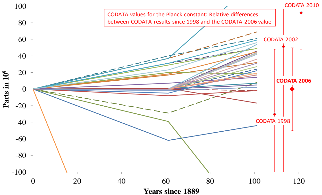
Figure 8. Mass changes of the six official copies (dashed lines) and national prototypes nos. 2 to 55 against the IPK since 1889 [18], compared with relative changes of CODATA values for the Planck constant, h , since 1998 [5, 12, 13], where the CODATA 2006 value was (arbitrarily) chosen as a reference value.
