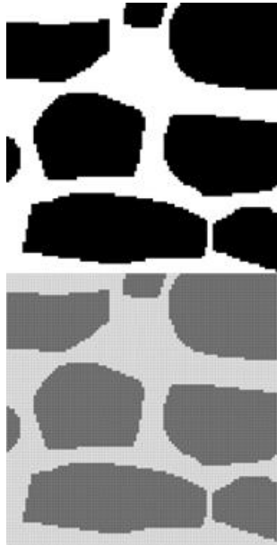
Fig. 1. Rasterized sketch of sample masonry panel (top); resulting 2D finite element mesh (bottom).
