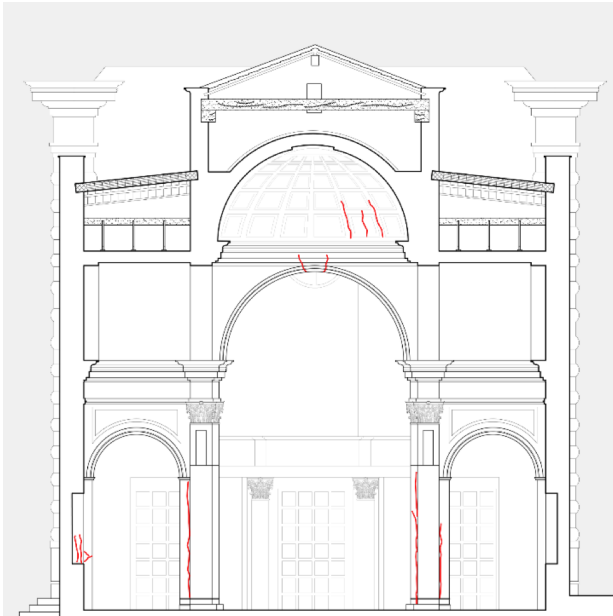
Fig.6. Transverse section with cracks survey
