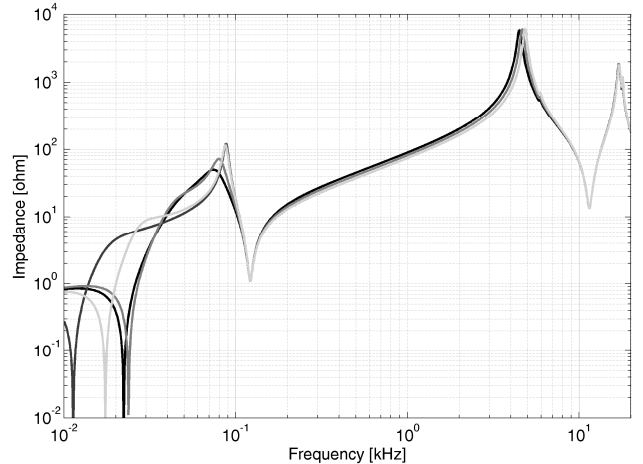
Fig. 3. Sensitivity analysis of Z_p for varying vehicle input filter: E402B, E412, TAF, ETR460 (see Table 1).
