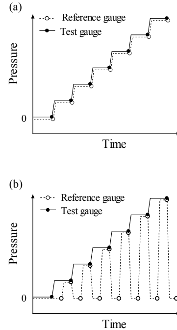
Fig. 3. Pressurization procedures for reference and test gauges during calibration: conventional method (a), and proposed method (b). For both procedures, the test gauge is calibrated with a stepwise pressurization.
