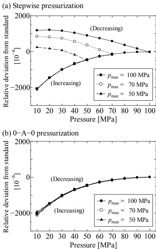
Fig. 2. Examples of calibration results for an electromechanical pressure gauge with the three maximum pressures, 50 MPa, 70 MPa, and 100 MPa. (a) Stepwise pressurization, (b) 0-A-0 pressurization.
