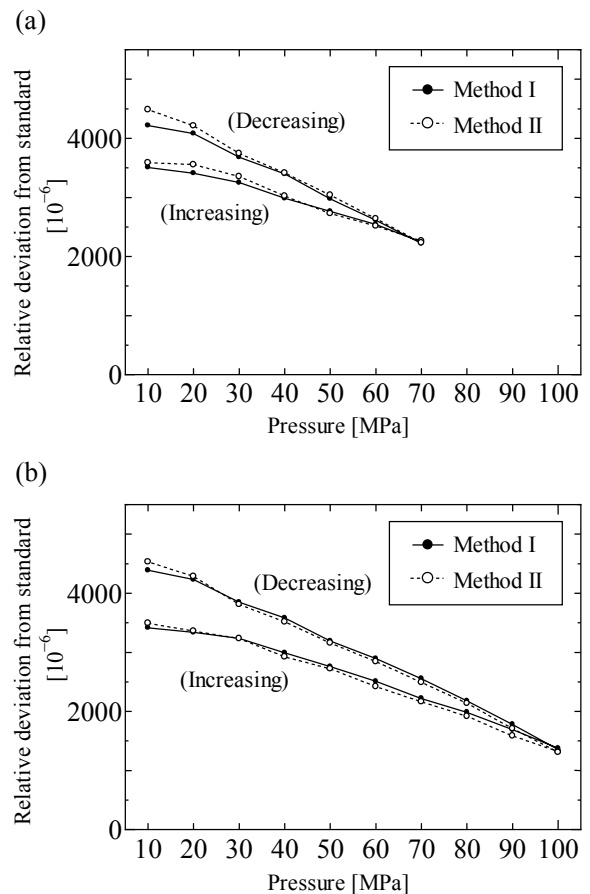
Fig. 5. Calibration results for the gauge B in demonstration experiment with (a) p_{max} = 70 MPa and (b) p_{max} = 100 MPa.
