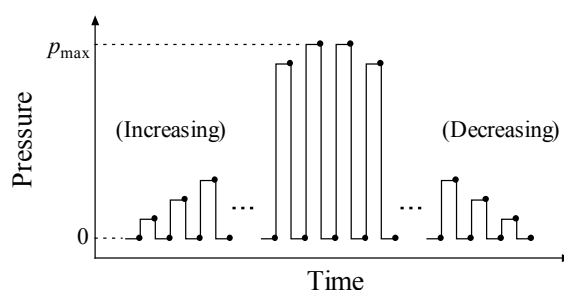
Fig. 1. Pressurization procedure for pressure gauge calibrations. (a) Stepwise pressurization, (b) 0-A-0 pressurization.
