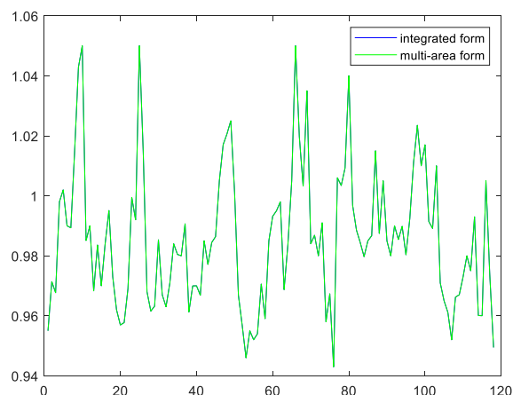
Figure 7. Comparison of voltage magnitudes in integrated and multi-area forms.
